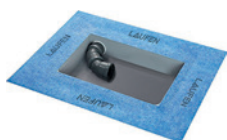
LAUFEN PRO H290041 Mounting box left for Marbond shower trays type DN 50 / height 100 mm, siphon not included
