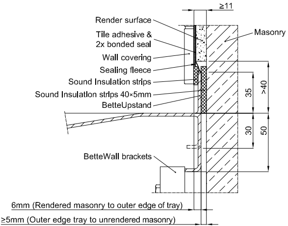
installation on solid wall
