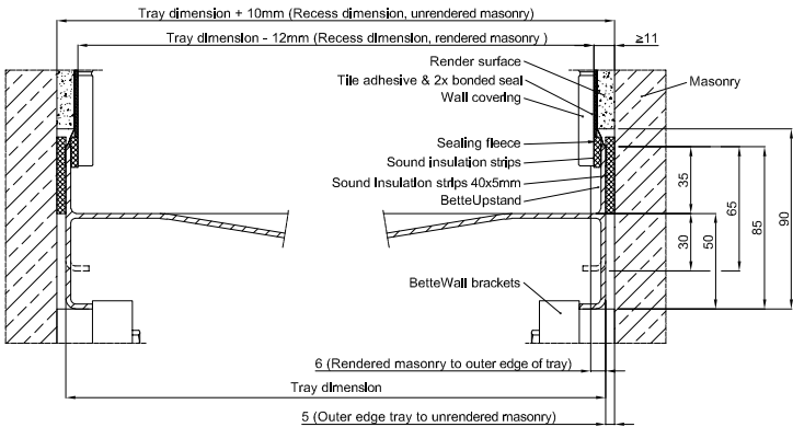
installation on solid wall
