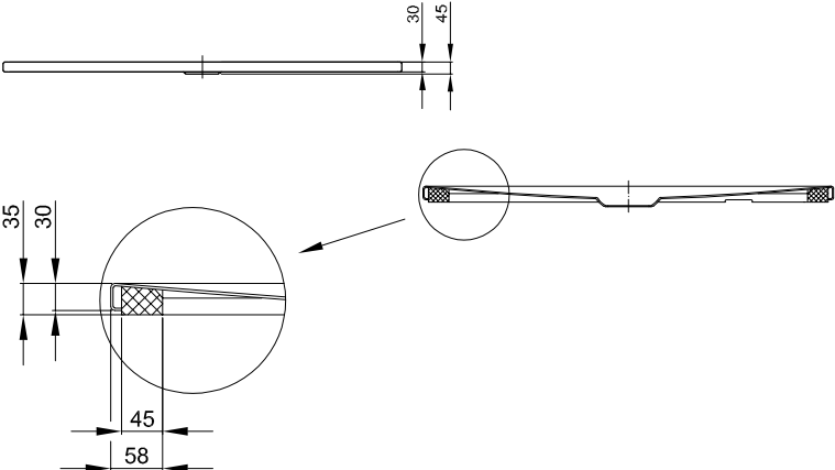
Illustration with pre-assembled Minimum support (T1).
