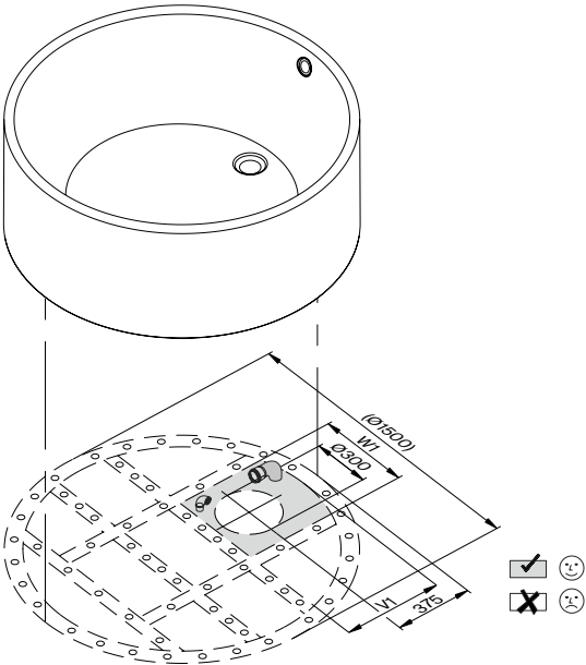
Adequate position to connect the drainage
