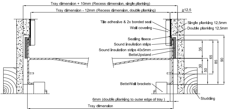
installation on dry wall
