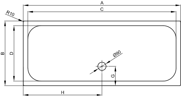
shower trays with dimension ≥ 1600 mm are delivered with waste positioned in centre of long shank.
