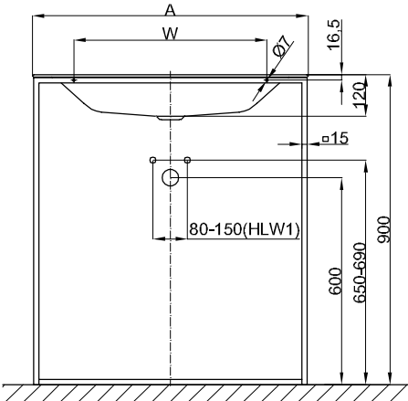
Dimensions for installation and connection:
