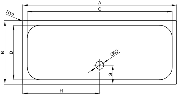
shower trays with dimension \geq 1600 mm are delivered with waste positioned in centre of long shank.
