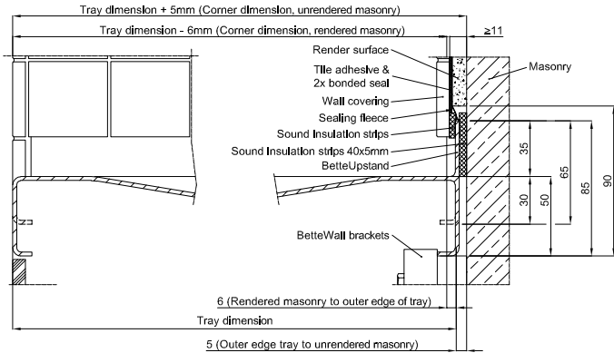
installation on solid wall
